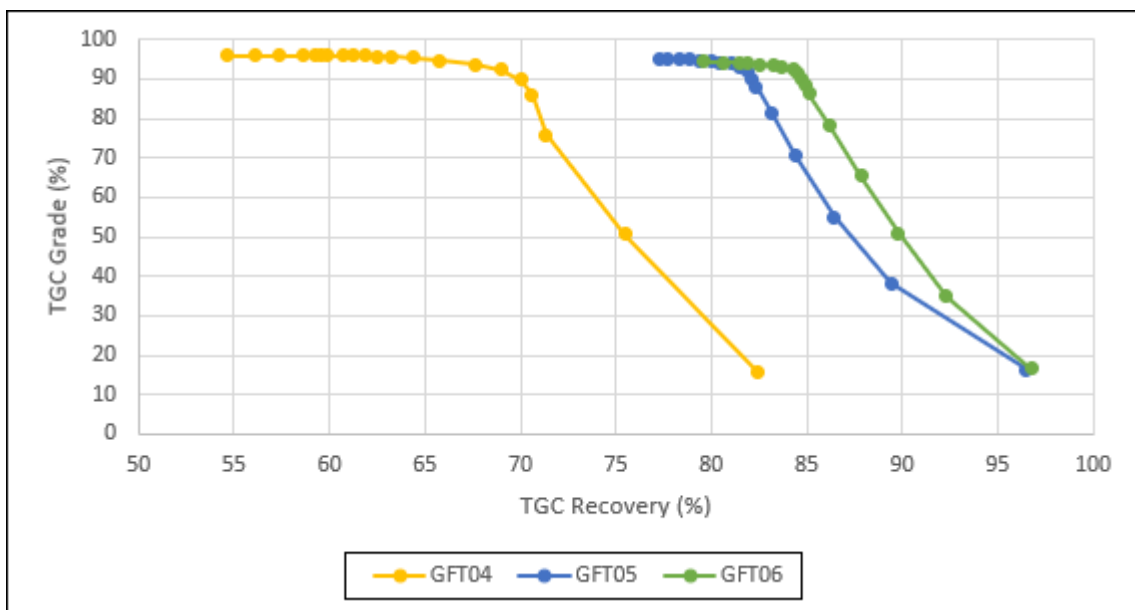
Figure 3: TGC Grade Recovery Profiles
